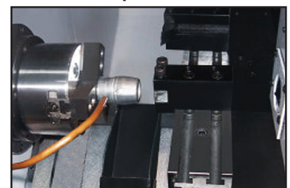
Step 4: Part catcher device comes to unloading device
