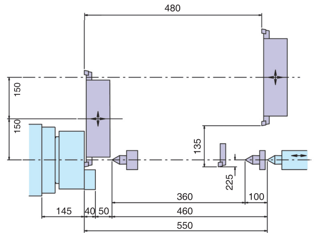
TNC - 08N (With tailstock)
